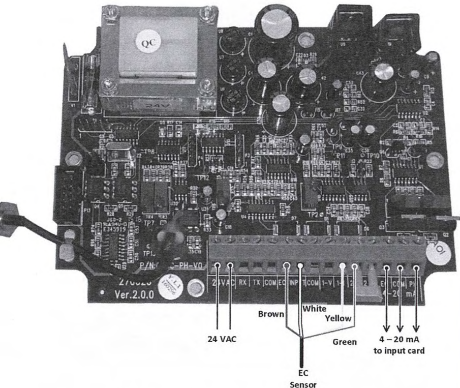
Figure 3: EC&pH Transmitter Wiring for EC Sensor (PT-100)
